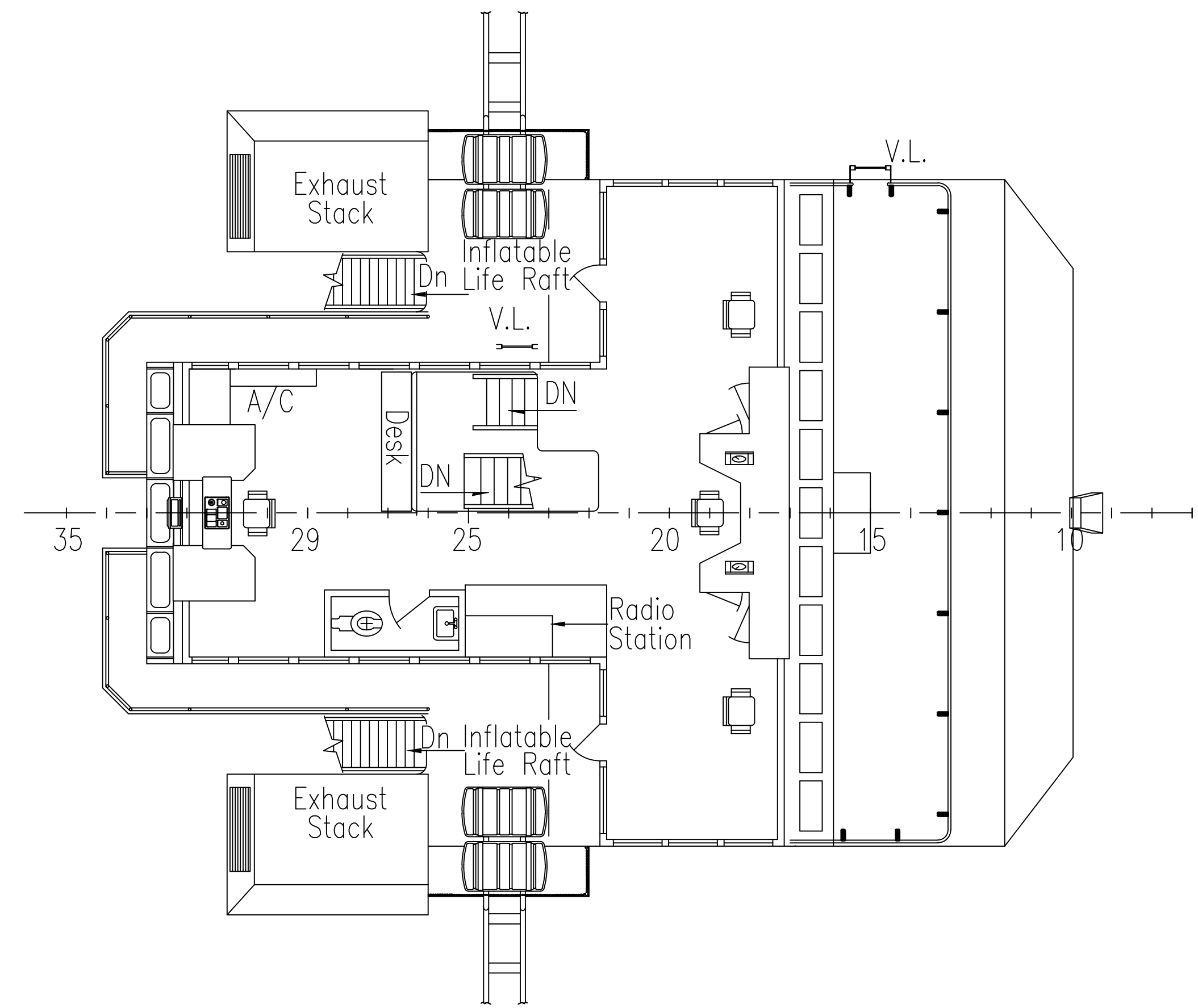
BRIDGE DK LEVEL 41'-10" ABOVE BASELINE
