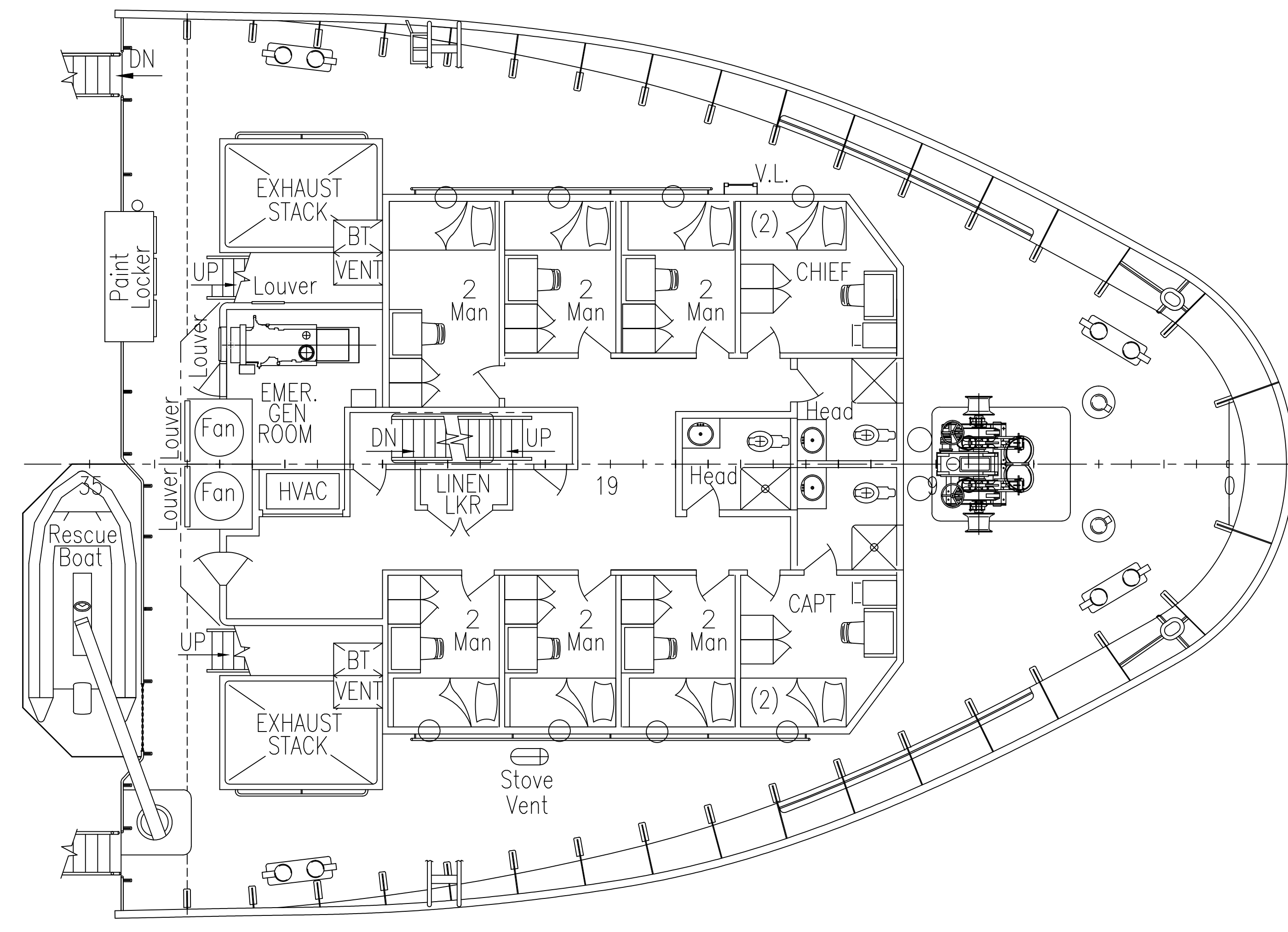
FOCSLE DECK 28'-0" ABOVE BASELINE
